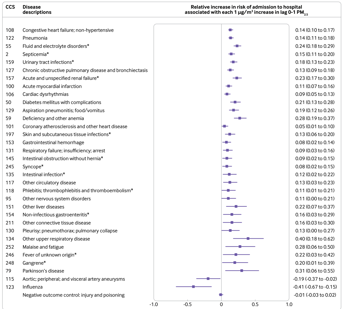
Fig 3 | Main analysis showing relative percentage increases in risk of hospital admission associated with each 1 \mu\text{g}/\text{m}^3 increase in lag 0-1 \text{PM}_{2.5} . Disease groups are ranked from highest to lowest absolute increase in risk of hospital admission. The main analysis was conducted in the case crossover study setting with lag 0-1 \text{PM}_{2.5} as the exposure, adjusted for penalized splines of lag 0-1 air and dew point temperatures for each disease group. The Bonferroni correction was used to adjust 95% confidence intervals for disease groups associated with lag 0-1 \text{PM}_{2.5} and negative outcome control (injury and poisoning). CCS=Clinical Classification Software code. *Indicates newly identified disease groups. Figure S2 in the supplementary online contents provides results for each of the 214 disease groups
